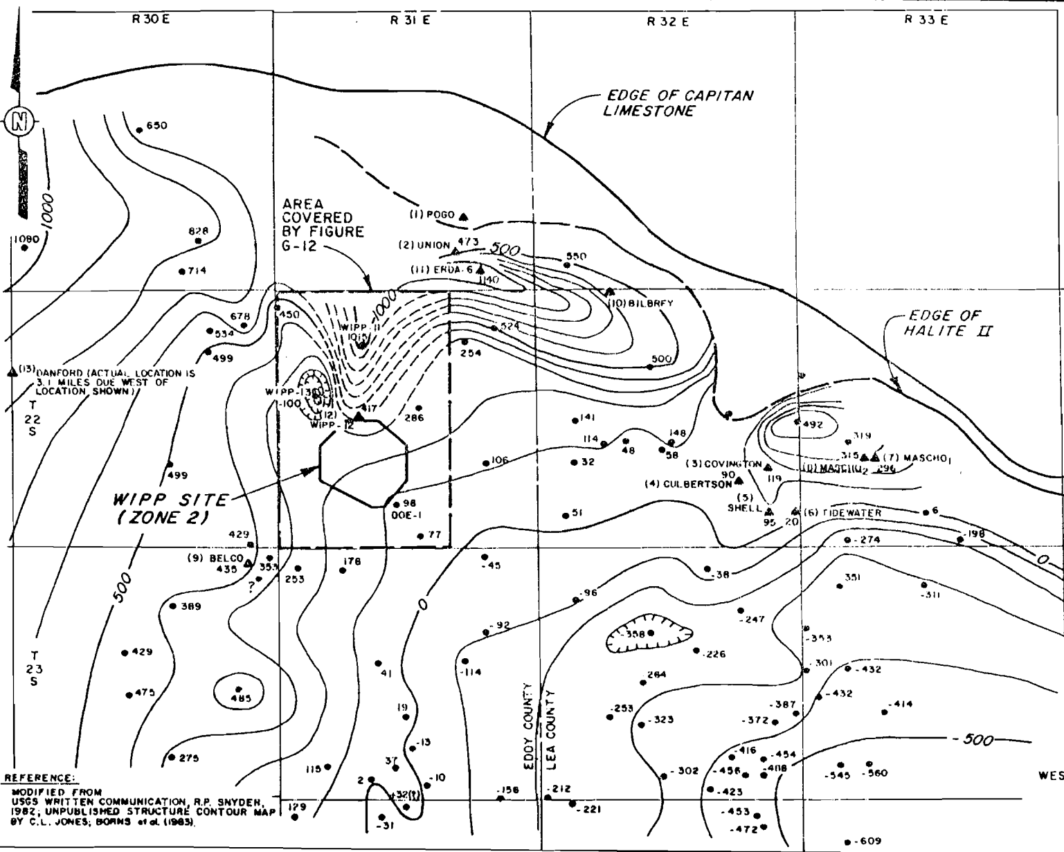
FIGURE G-11 STRUCTURE CONTOUR MAP OF NORTHEASTERN DELAWARE BASIN SHOWING BRINE OCCURRENCES PREPARED FOR WESTINGHOUSE ELECTRIC CORPORATION ALBUQUERQUE, NEW MEXICO
