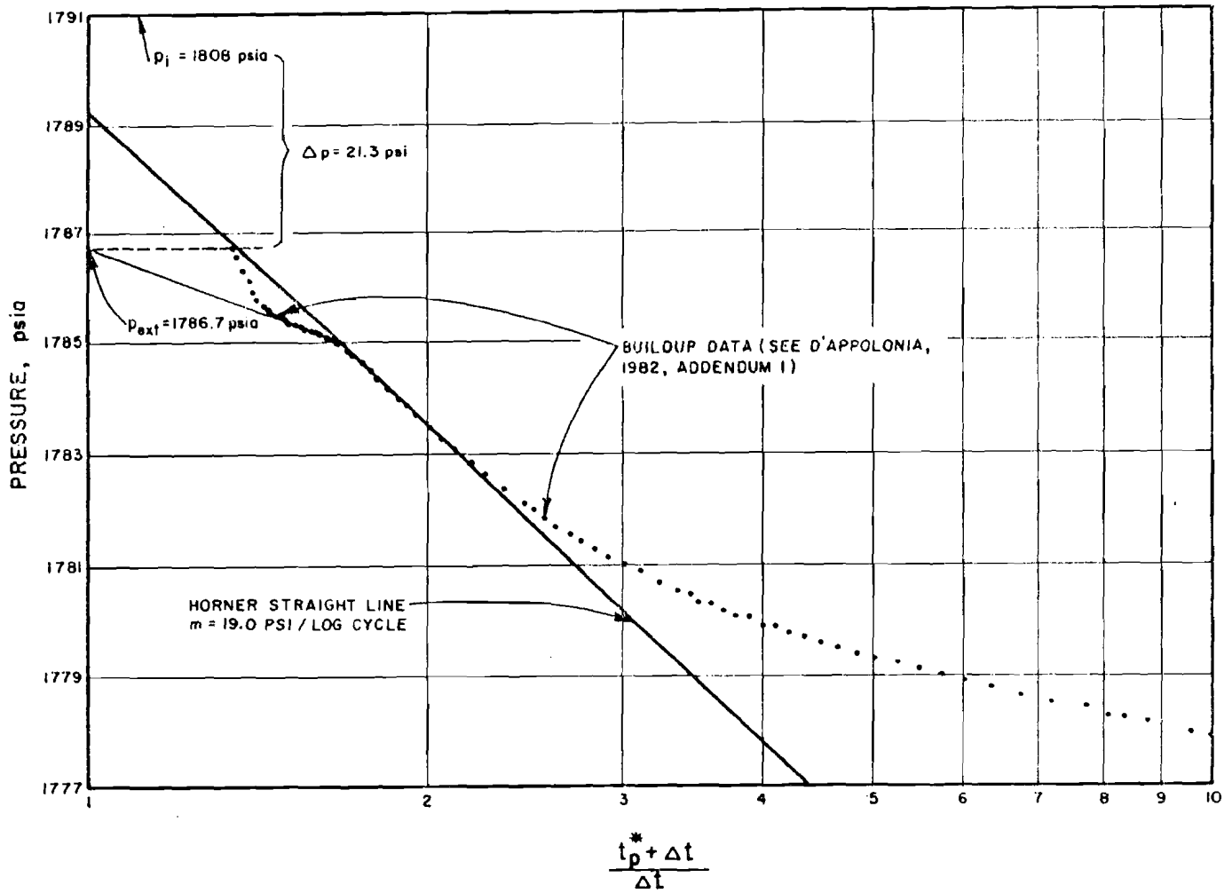
FIGURE H-5 HORNER PLOT OF WIPP-12 / FLOW TEST 2 / BUILDUP PERIOD DATA PREPARED FOR WESTINGHOUSE ELECTRIC CORPORATION ALBUQUERQUE, NEW MEXICO D'APPOLONIA
