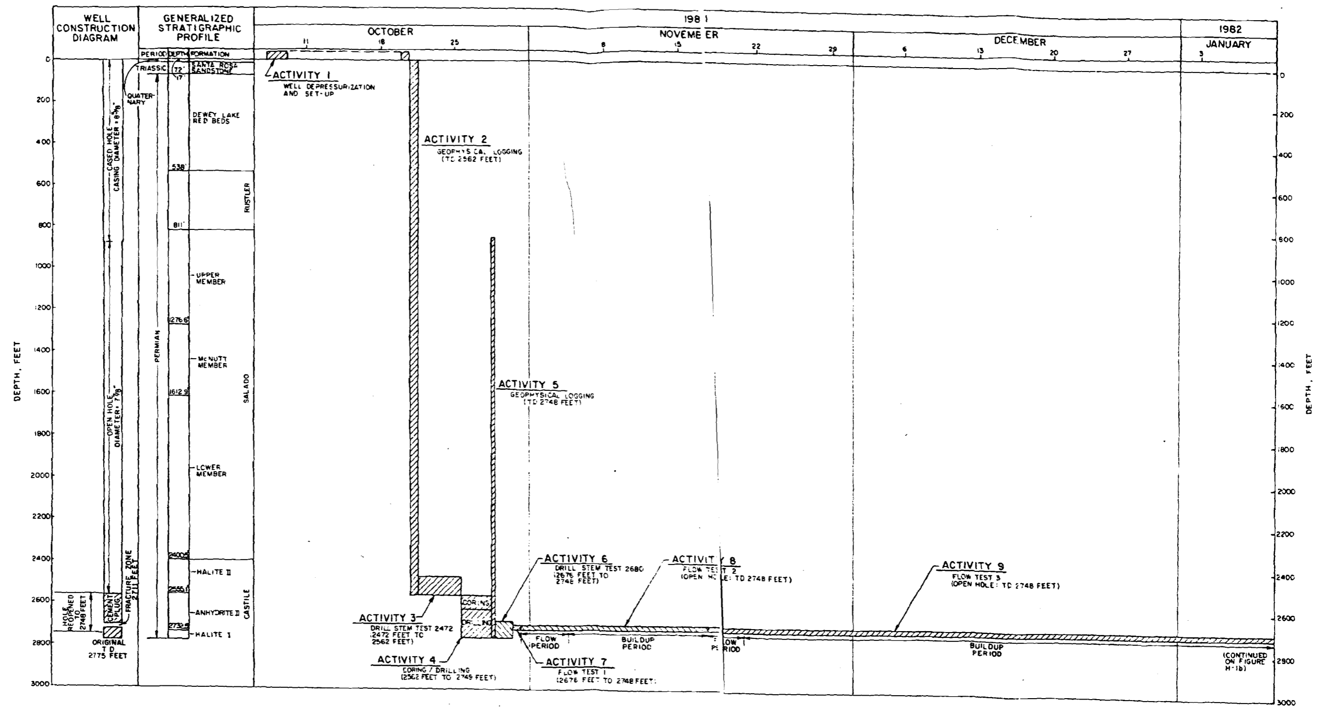
FIGURE H-1a ERDA-6 TIME-VERSUS-DEPTH ACTIVITY SUMMARY PREPARED FOR WESTINGHOUSE ELECTRIC CORPORATION ALBUQUERQUE, NEW MEXICO
