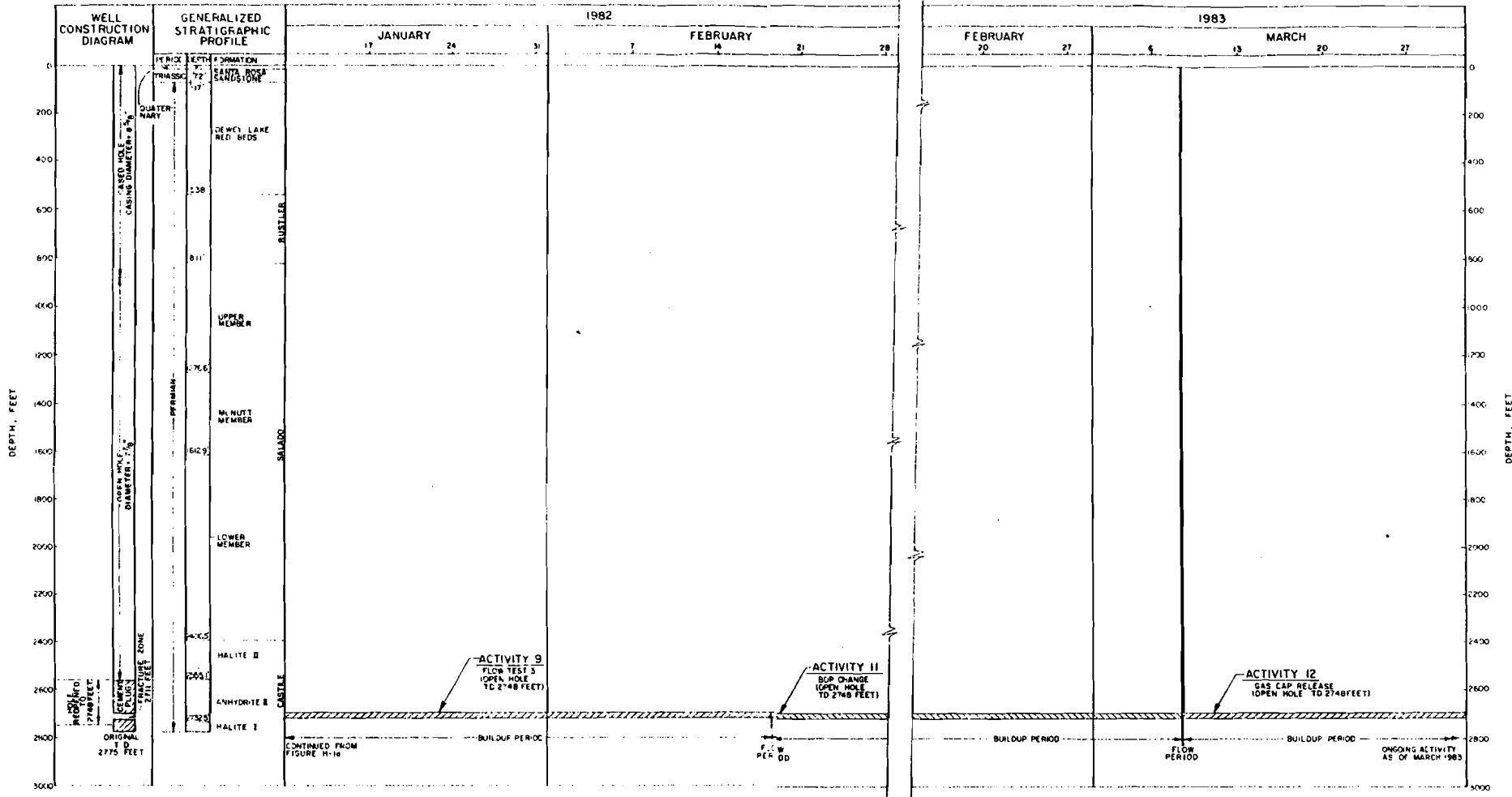
FIGURE H-1b ERDA-6 CONTINUATION OF TIME-VERSUS-DEPTH ACTIVITY SUMMARY
