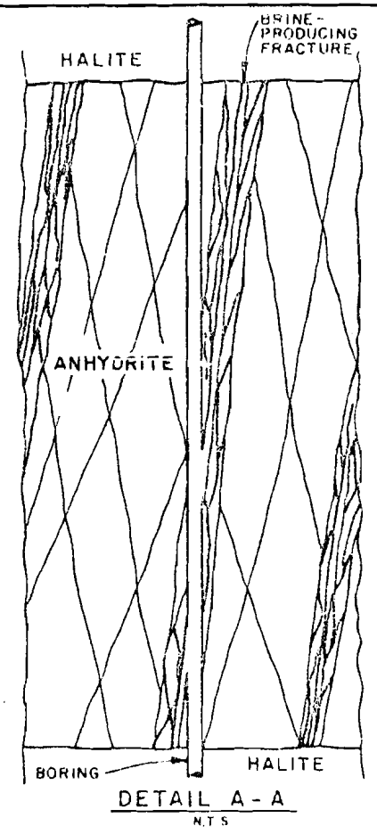
FIGURE G-13 SCHEMATIC OF BRINE RESERVOIR FORMATION PREPARED FOR WESTINGHOUSE ELECTRIC CORPORATION ALBUQUERQUE, NEW MEXICO
