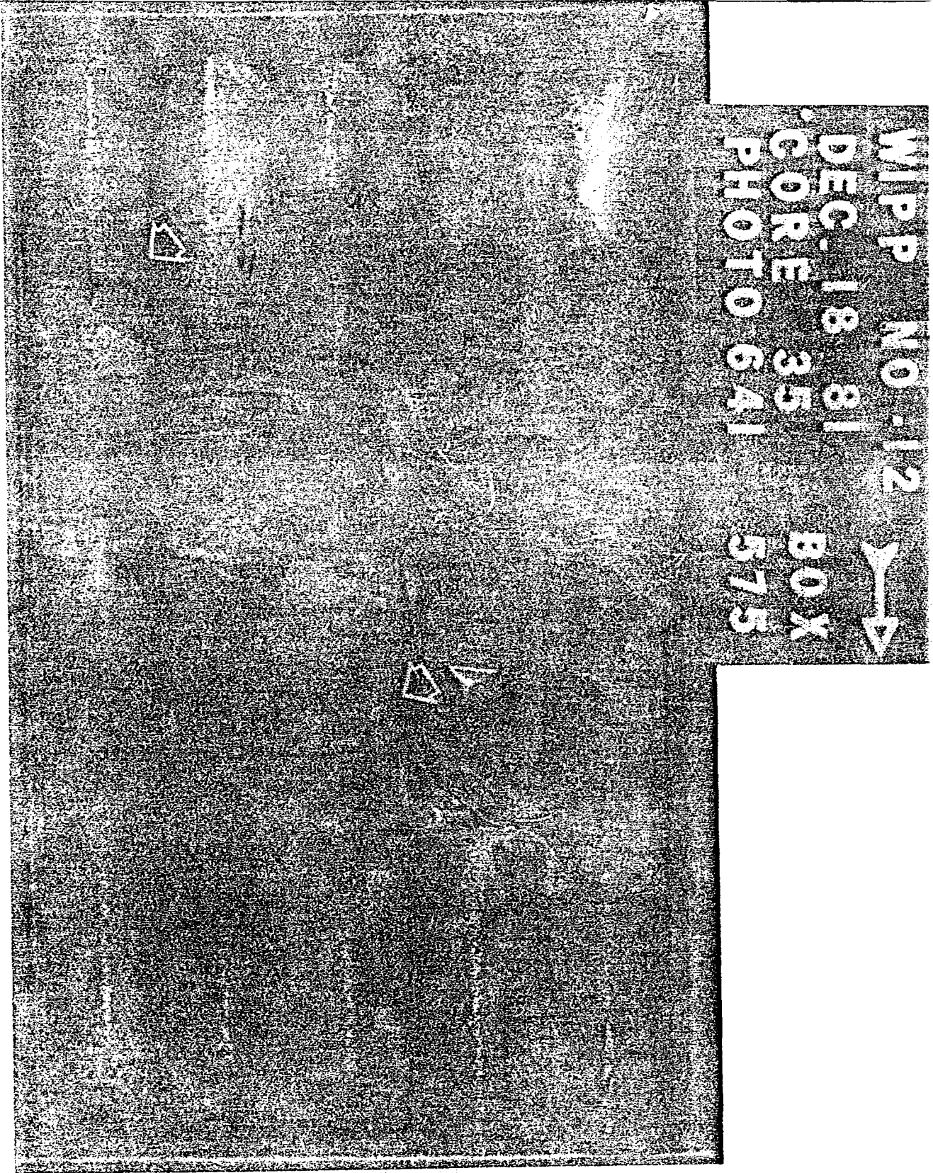
FIGURE G-8 EXAMPLE OF MICROFOLDING STYLE IN HALITE II PREPARED FOR WESTINGHOUSE ELECTRIC CORPORATIO ALBUQUERQUE, NEW MEXICO D'APPOLONIA
