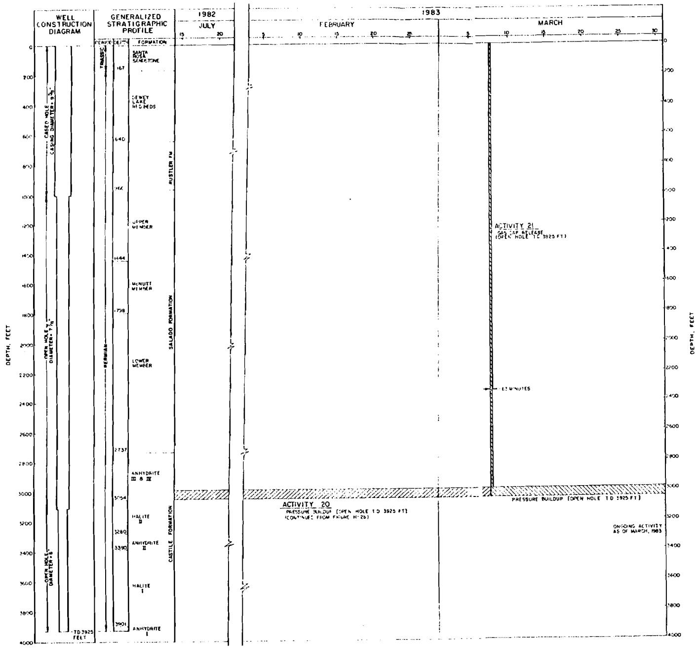
FIGURE H-2c WIPP-12 CONTINUATION OF TIME-VERSUS-DEPTH ACTIVITY SUMMARY PREPARED FOR WESTINGHOUSE ELECTRIC CORPORATION ALBUQUERQUE, NEW MEXICO D'APOLLONIA
